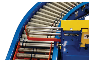
Horizontal Side Stop
